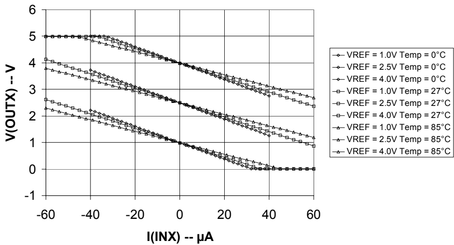
DC-Transfer-Curve V(OUTX) = f(I(INX)) -- R_f = 25k\Omega
